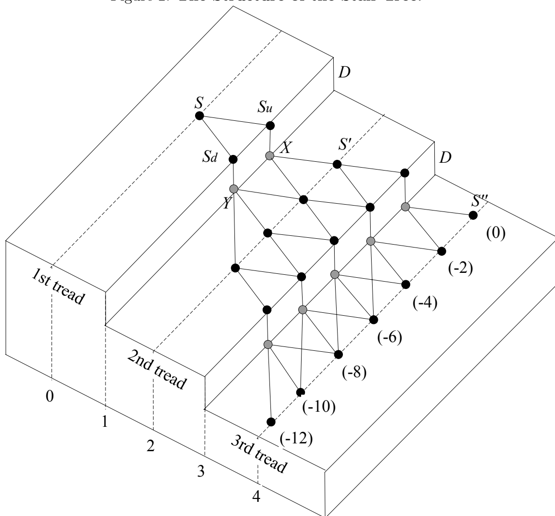
Figure 2: The Structure of the Stair Tree.
