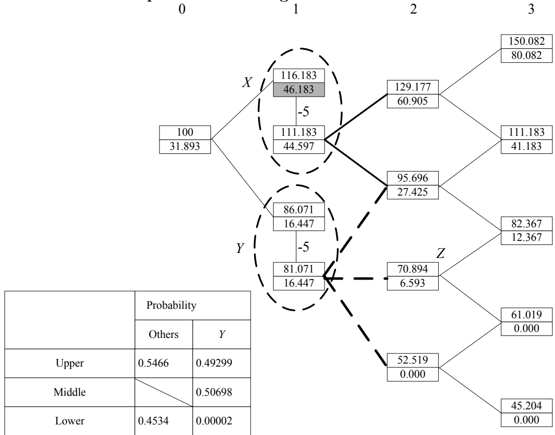
Figure 4: A 3-Time-Step Tree for Pricing an American Vanilla Call.
