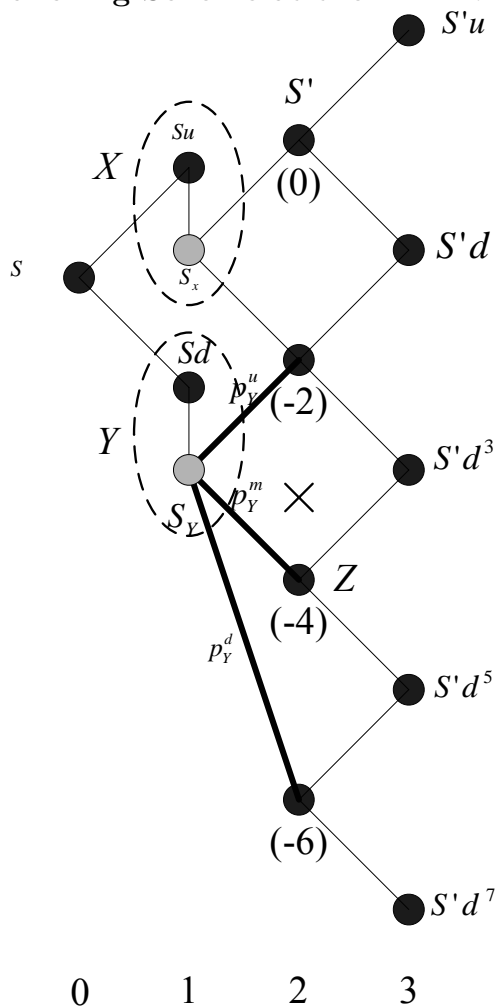
Figure 3: Branching Scheme at the Ex-Dividend Date.
