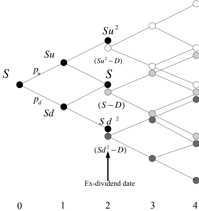
Figure 1: The Bushy Tree.
