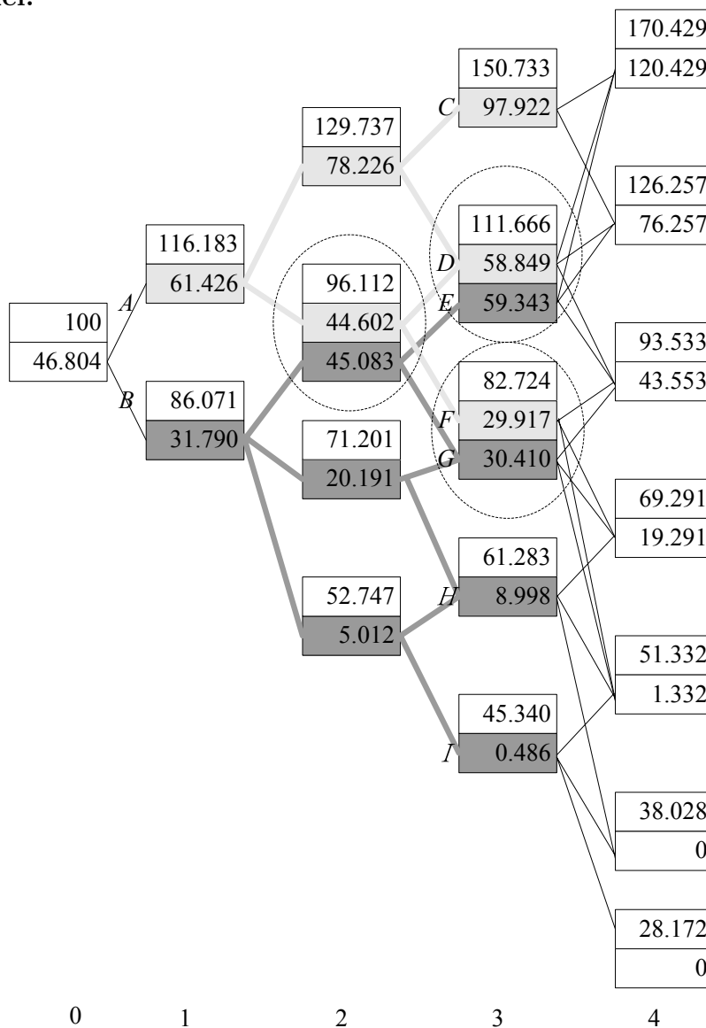
Figure 6: A 4-Time-Step Stair Tree that Incorporate the Marsh and Merton's Dividend Model.
